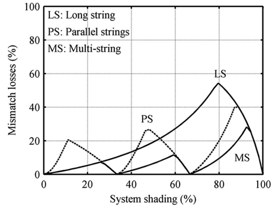
Fig. 8. Mismatch losses of the PV power generators under partial shading conditions as a function of system shading for shading strength of 85%.
