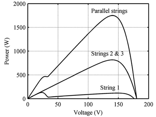
Fig. 13. P - U curve of the Parallel strings generator and individual curves of parallel-connected Strings 1, 2, and 3 under partial shading conditions with shading strength of 85% and with system shading of 26%.
