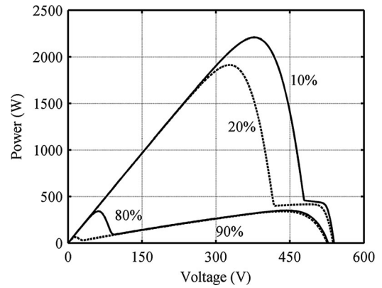
Fig. 11. P - U curves of the Long string generator under partial shading conditions with shading strength of 85% and with system shadings of 10%, 20%, 80%, and 90%.
